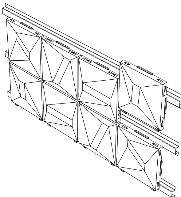
Mounting method for attaching tiles to aluminium profiles
