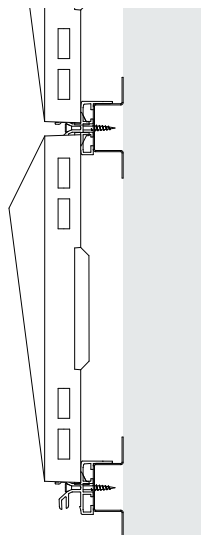
Mounting method for attaching tiles to aluminium profiles
